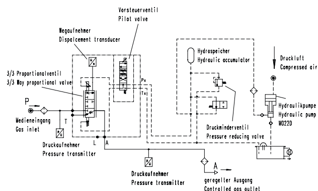
Figure: Block diagram control block with pilot control hydraulic supply
