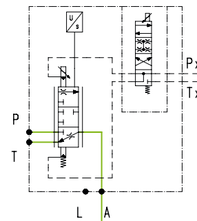
Figure: schematic diagram 3/3-Way Proportional Valve
