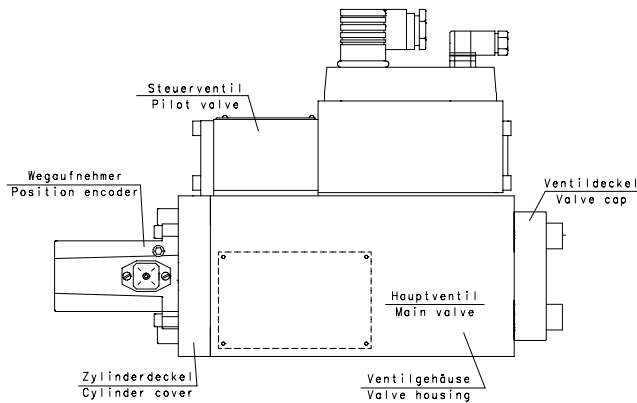
Figure: Assembly 3/3-Way Proportional Valve
