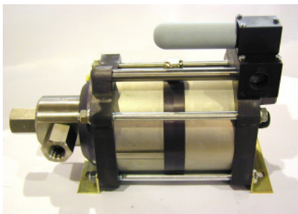
G35-2 (L) single acting, double air drive head (Standard= Bottom inlet)
